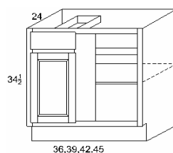
Base Blind Corner L/R BBC42-45
