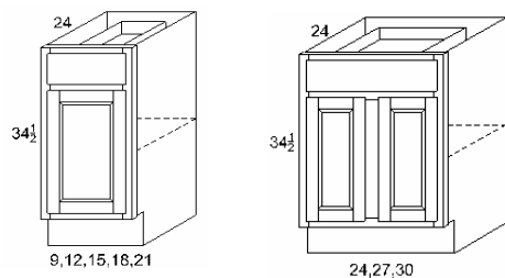
Base Cabinet 1 Drawer, 1 Door, 1 Shelf
